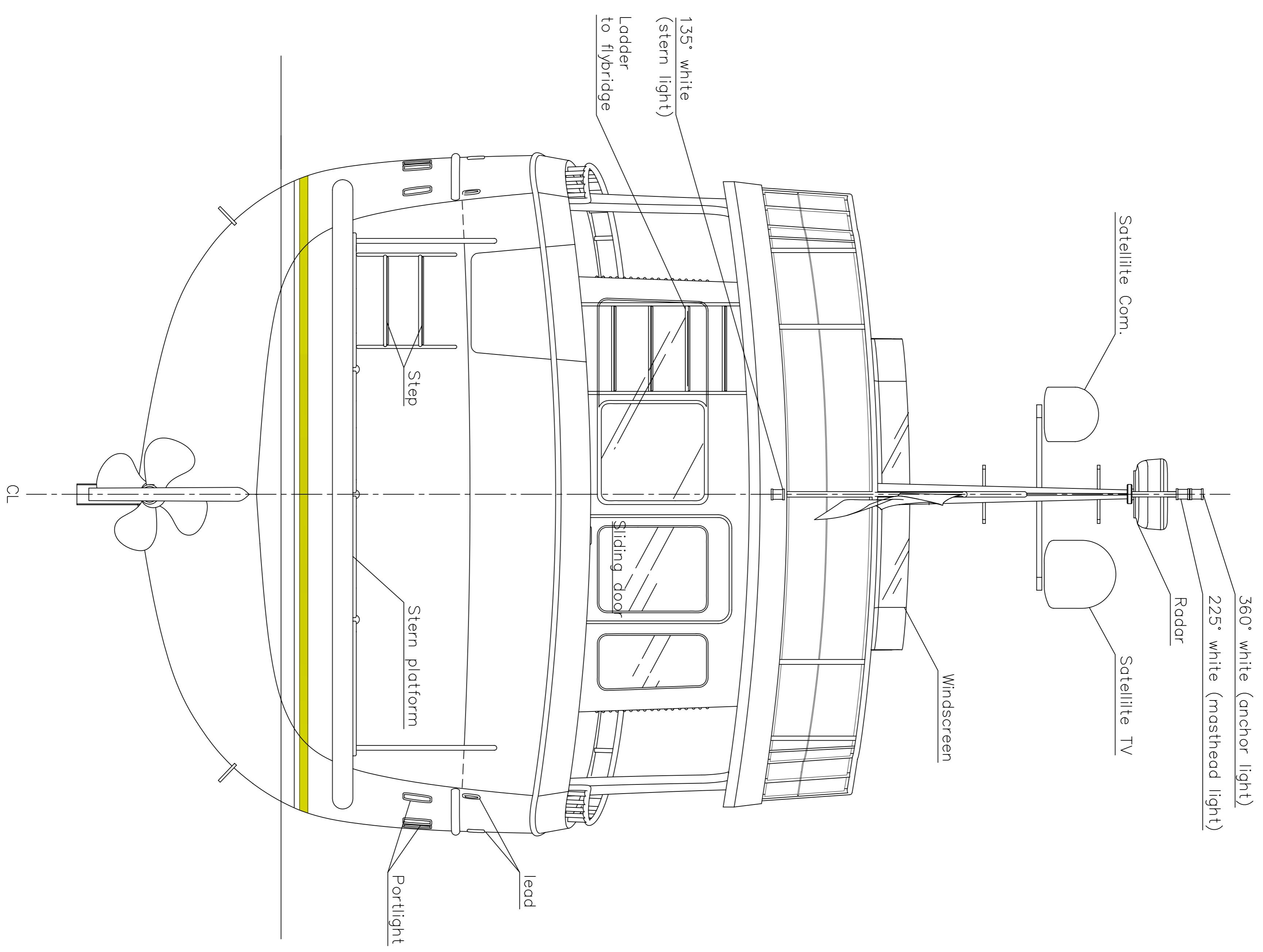
VIEW FROM STERN
